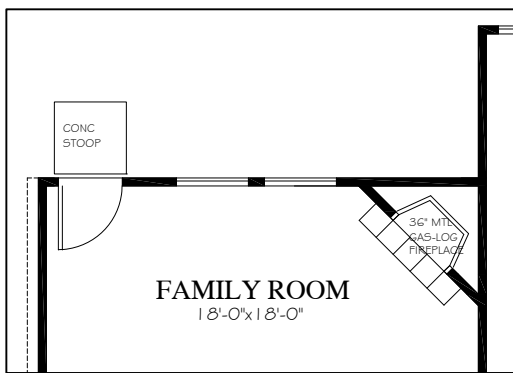
OPTIONAL FIREPLACE FAMILY ROOM
